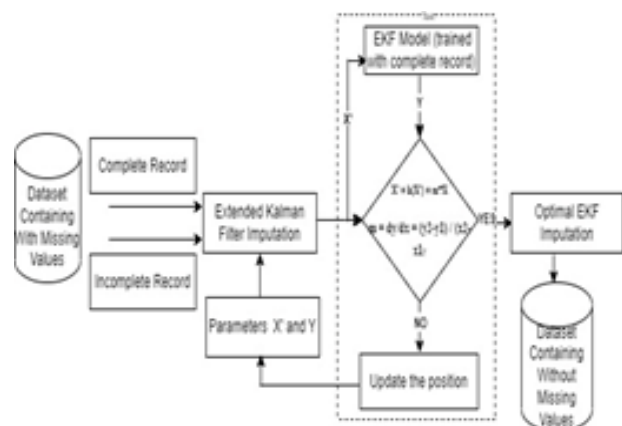
Figure 4: Process of extended Kalman for missing value imputation.
