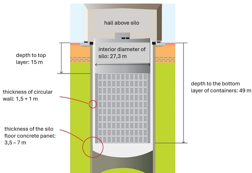
Figure 1: LILW disposal facilities in the form of a near-surface silo with an above-ground hall.
