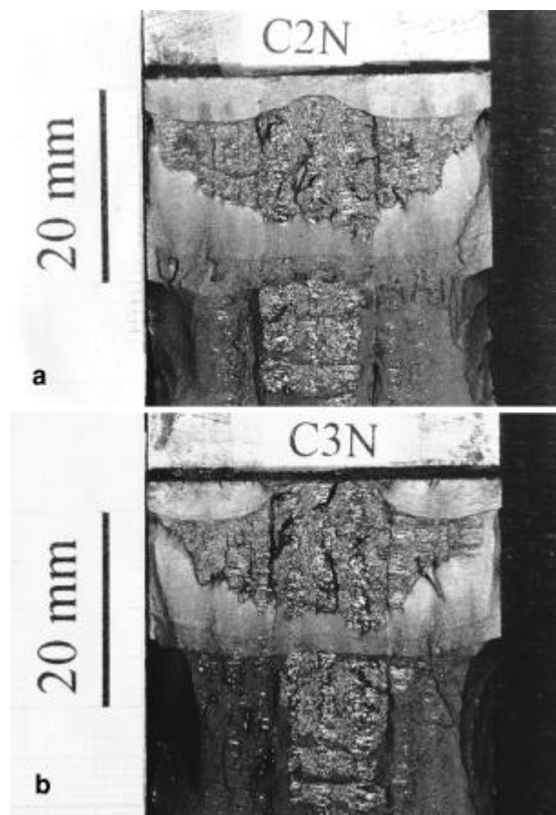
Figure 5: Obtained fatigue crack shapes through-the-thickness of specimen, a/W=0.5 ; W=72 \text{ mm} using a) low and b) high cycling fatigue under the effect of residual stresses
