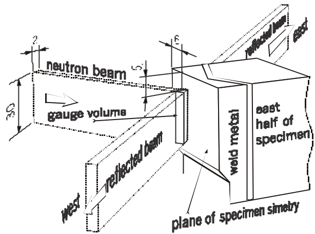
Figure 2: Position of gauge volume (2x2x30 mm) in the welded joint Slika 2: Polo{aj obsevanega volumna (2x2x30 mm) v zavarjenem spoju
