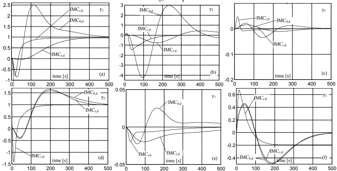
Fig. 6. Time responses of perturbed plant (44) to unity step signal:(a-b) in input u_1 ; (c-d) in input u_2 ; (e-f) in input d
