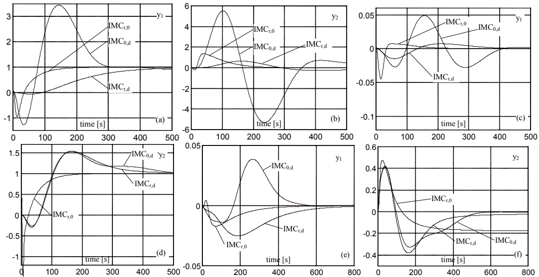
Fig. 7. Time responses of perturbed plant (45) to unity step signal: a,b) in input u_1 ; c,d) in input u_2 ; e,f) in input d
