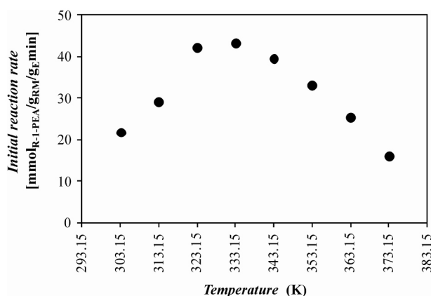
Figure 9. Influence of temperature on initial reaction rate for acylation of ( R,S )-1-phenylethanol with vinyl acetate in [bmim][BF 4 ]. Reaction conditions: 5.0 mmol ( R,S )-1-phenylethanol, 5.0 mmol vinyl acetate, 5.0 mmol [bmim][BF 4 ], 100.4 \text{mg}_E/\text{g}_{\text{RM}} immobilized CALB, 600 rpm, 5 h of reaction performance.
