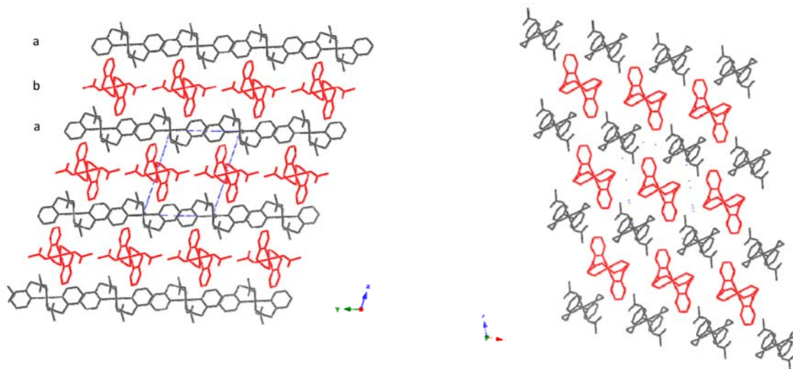
Figure 5. Packing diagram of 1 viewed along a axis (left) and b axis (right) illustrating different relative arrangement of two types of \text{Ni}(\text{ac})_2(2\text{-PyEtOH})_2 molecules.
