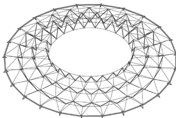
Slika 4: Oblika konstrukcije nateznikov s središčno odprtino. Figure 4: Shape of the tension-strut crystal structure with central opening.
