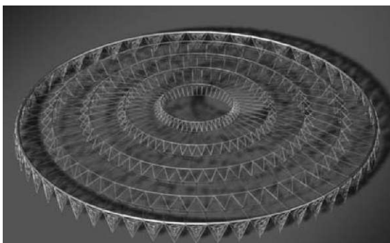
Slika 6: Pogled na celotno konstrukcijo objekta Hall 2010. Figure 6: Overall view of the structure Hall 2010.
