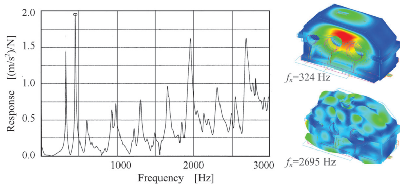
Fig. 10. Modal responses of the housing; a) response measured at point MT0 due to excitation at point T1, b) some of excited modal shapes obtained numerically
