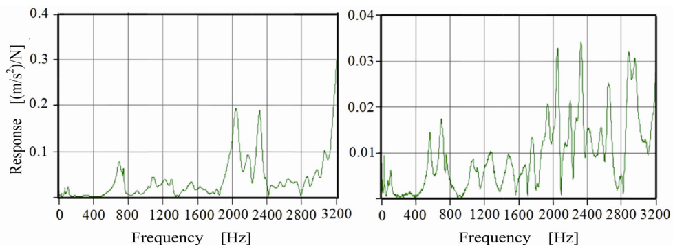
Fig. 11. Comparison of the results of modal tests of the housing with the gear system; a) excited by the impact inside the bearing hole in the direction of the gear contact line, b) excited by the impact at the tooth addendum of the middle gear
