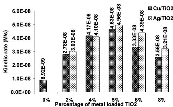
Fig. 11: Kinetic rate of degradation of SA for pure TiO 2 and five concentration of metal coated TiO 2 at 85 °C
