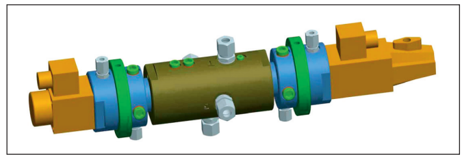
Figure 2. 3D model of a functional prototype of a proportional 4/3 directional sliding control valve
