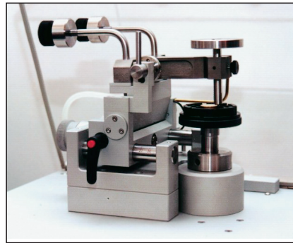
Figure 6. Pin-on-Disc wear tester (CSEM)
