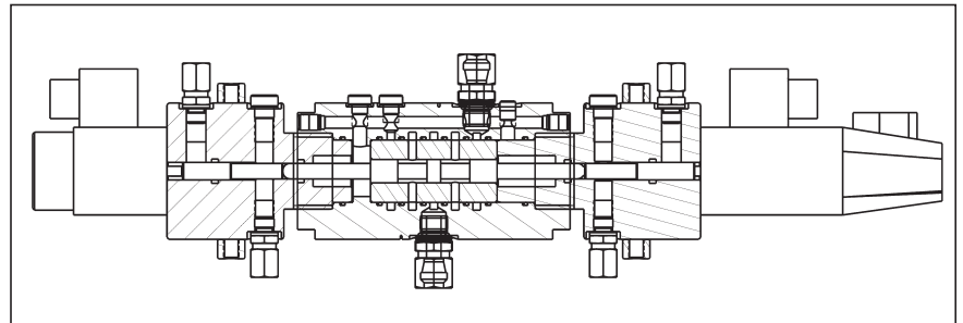
Figure 3. Cross section of the functional prototype of a proportional 4/3 directional sliding control valve
