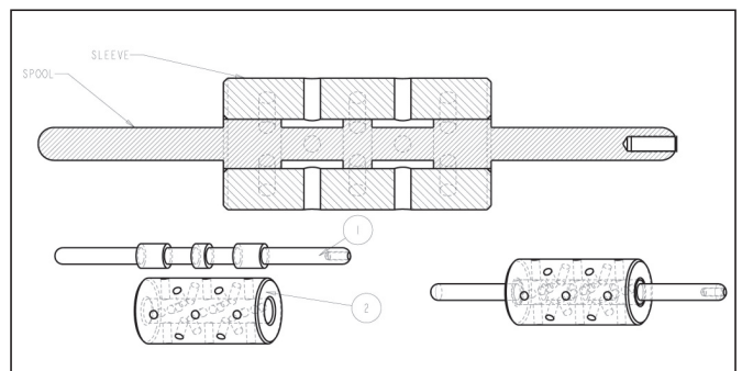
Figure 4. Main parts of the specimen: 1) spool and 2) sleeve
