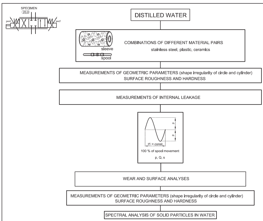
Figure 5. Course of life-time measurement on the main test rig
