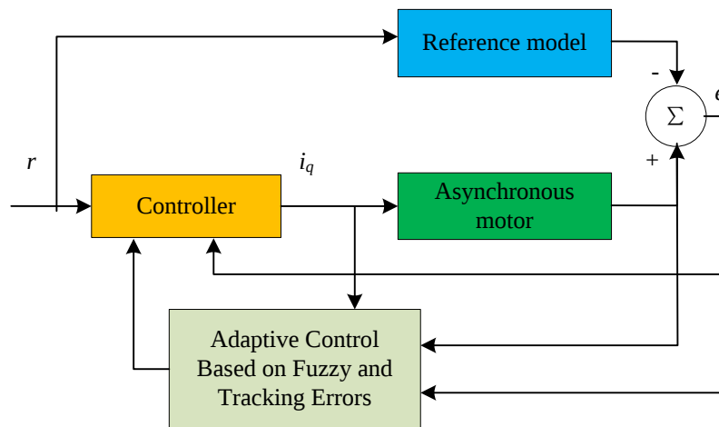
Figure 4: Controller structure
