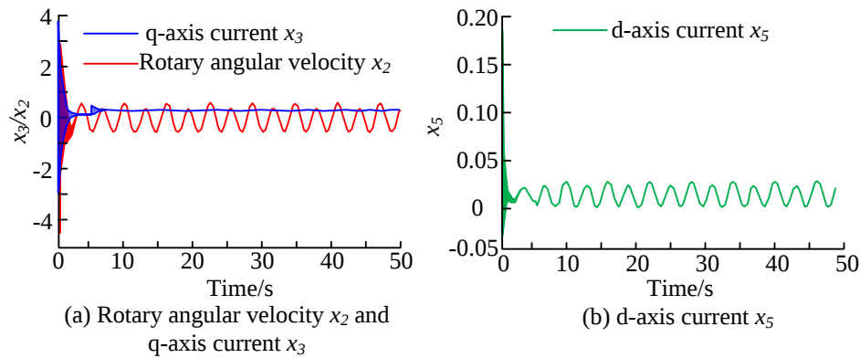
Figure 9: Rotor angular velocity x_2 , q-axis current x_3 , and d-axis current x_5 of an asynchronous motor system
