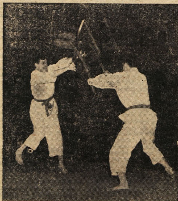
Z nastopa pripadnikov LM v Trbovljah Karli SAURIC
