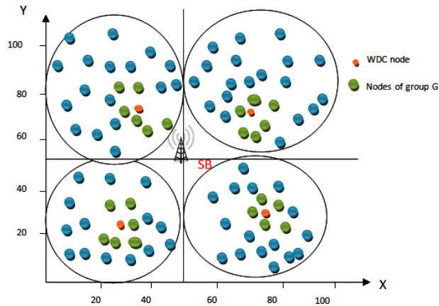
Figure 4: WDC calculation.
