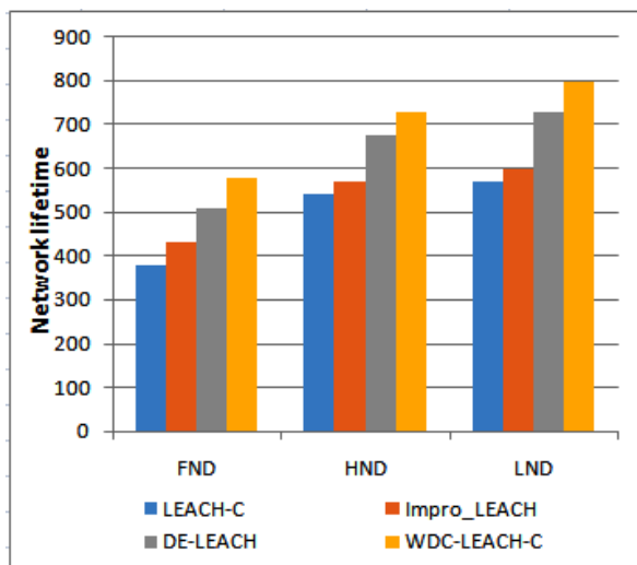
Figure 7: Network lifetime.
