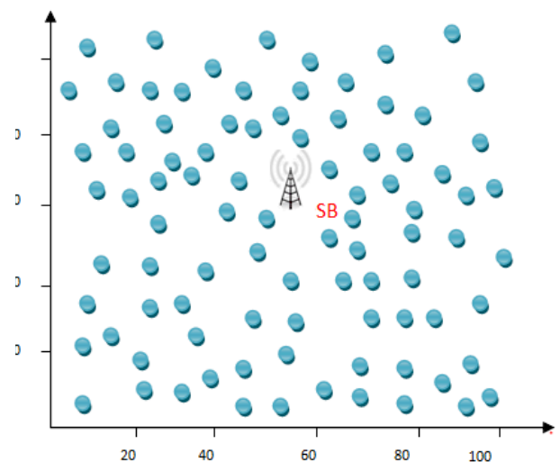
Figure 1: Network Model.
