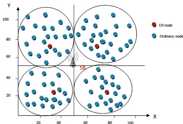
Figure 5: CH selection.
