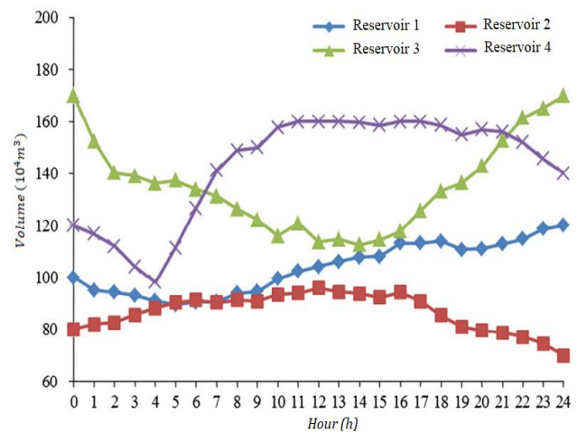
Figure 5: Ideal reservoir storing standards of case 1.
