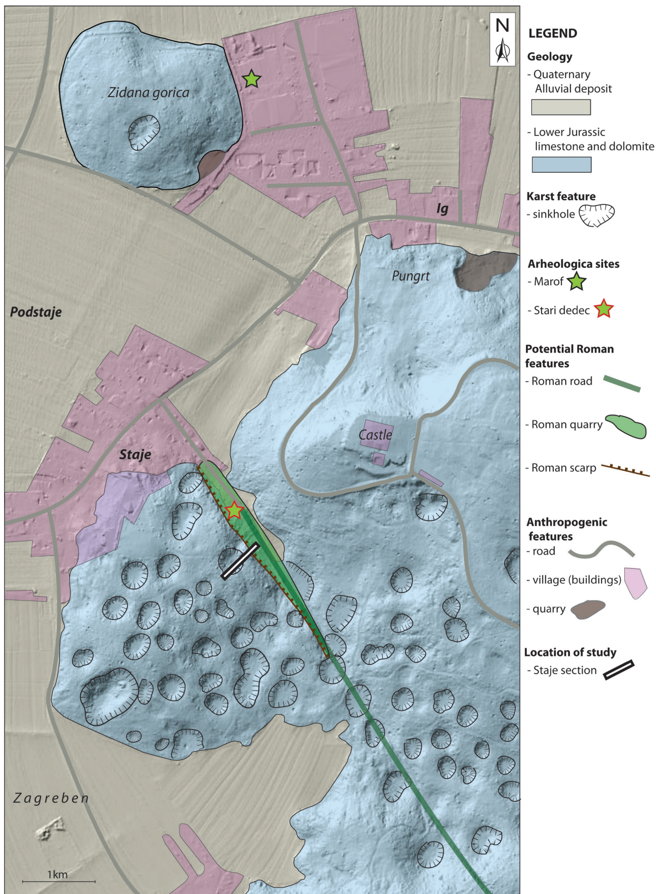
Fig. 2. Geomorphological map of the area of Staje and Marof with marked positions of the logged section (potential roman quarry), “Stari dedec” Roman monument and Marof archeological site.
