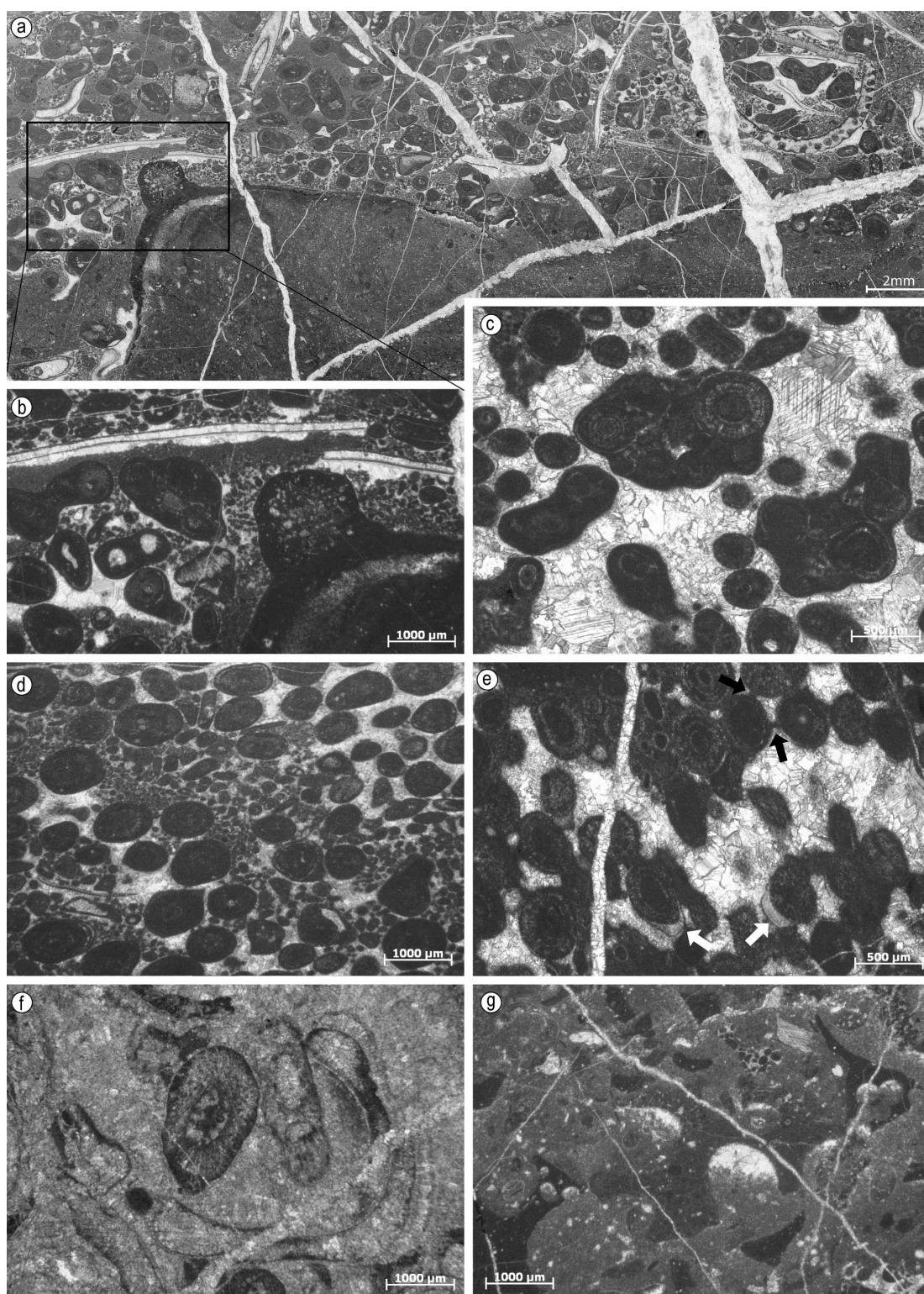
Fig. 8. Microfacies of calcarenite, lumachella and lithoclastic microbreccia.
