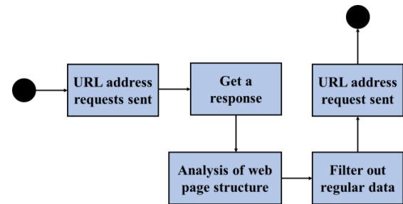
Figure 3: Page crawl flow chart.
