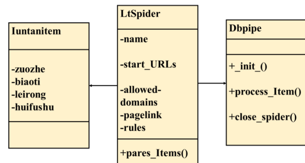
Figure 4: Page crawler diagram.
