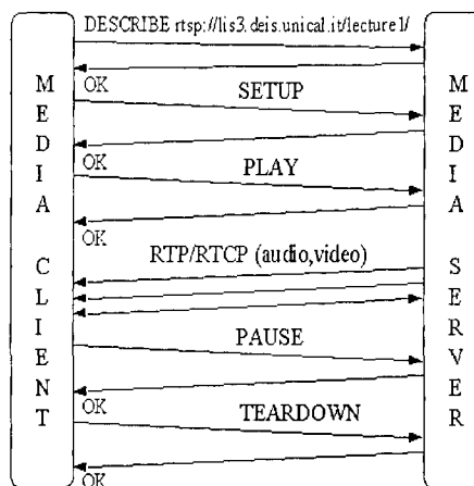
Figure 3: RTSP playback session example
