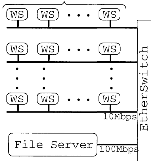
Figure 4: Workstation cluster for evaluations.
