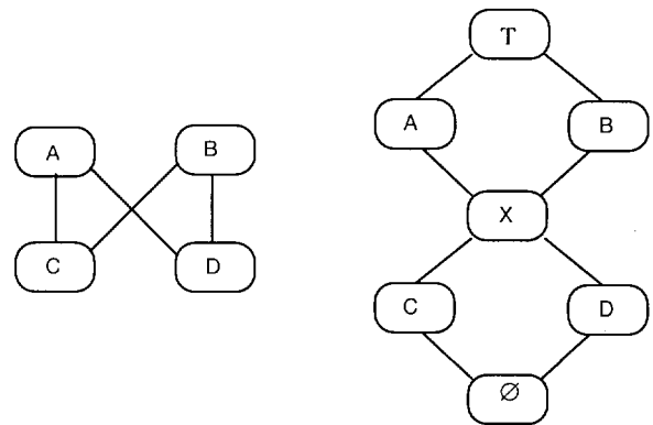
Figure 2: (left) A poset representation of the class S of Fig. 1. (right) The normal completion of the poset to the left.
