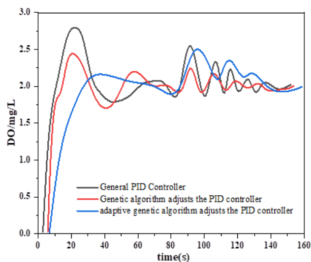
Figure 6: Comparison curve of anti-interference simulation.
