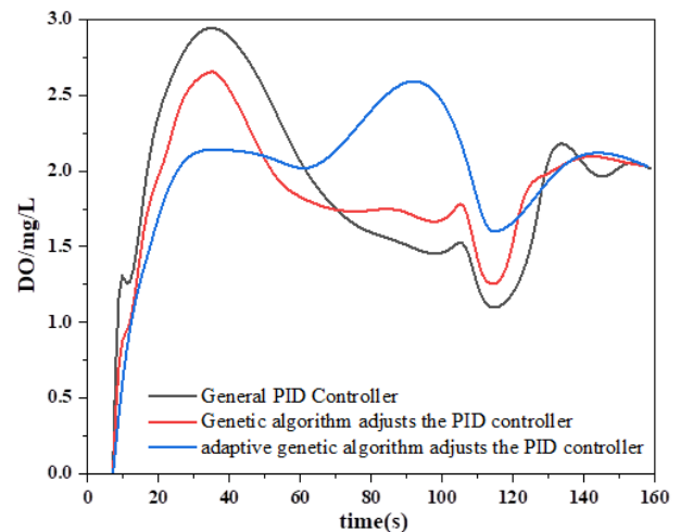
Figure 7: Comparison curve of robustness simulation.
