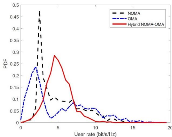
Figure 5: The user rate's PDF for NOMA, OMA, as well as Hybrid NOMA-OMA model
