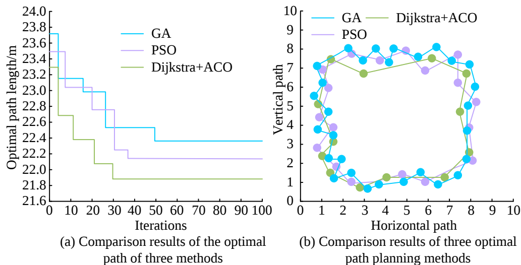
Figure 7: Comparison results of optimal path length and path planning using three methods
