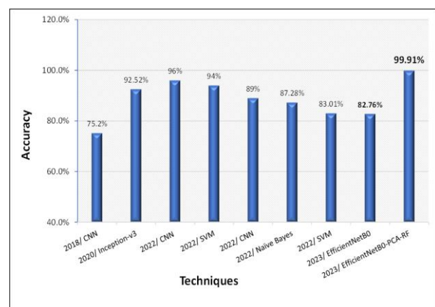
Figure 6: The comparison of the accuracy score of proposed methods with the previous studies
