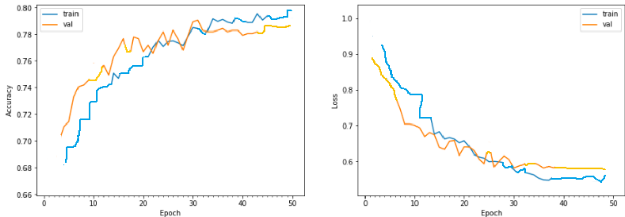
Figure 3: Model accuracy and loss.
