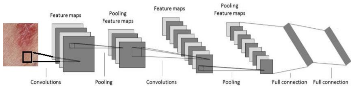
Figure 1: A typical architecture of a CNN Model.
