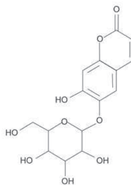
Figure 5: The chemical structure of aesculin [31]
