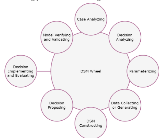
Figure 1: DSM Wheel [11]
