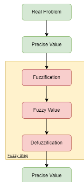
Figure 2: FL Algorithm
