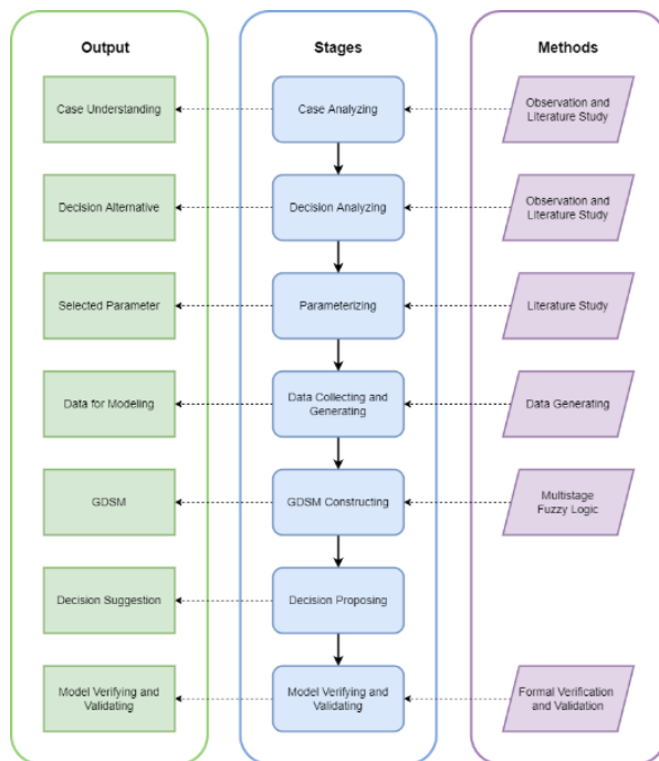
Figure 3: Research stages
