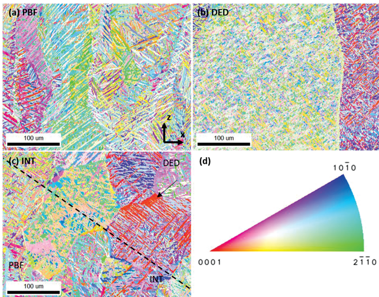
Figure 6: EBSD image of the (a) PBF, (b) DED (c) and INT part of the HAM sample. The dotted black line on (c) image show approximate location of the INT. The (d) image shows the inverse pole figure colour triangle for the \alpha phase
