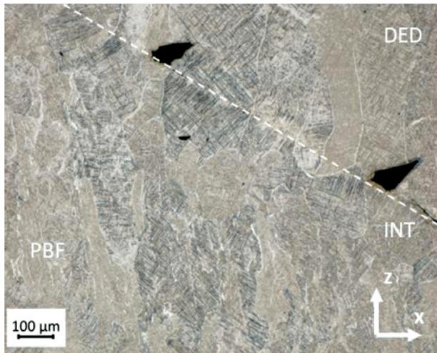
Figure 4: OM image of the microstructure at the INT between the PBF and DED technology of the HAM part
