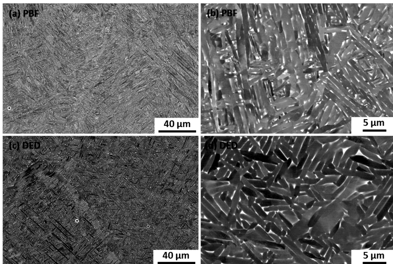
Figure 3: SEM-BEI of the microstructure in (a and b) PBF, (c and d) DED part of the HAM sample
