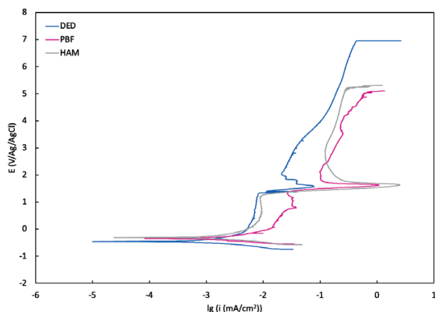
Figure 8: Potentiodynamic curves for DED, PBF and HAM Ti6Al4V alloy in 3.5 % NaCl solution.
