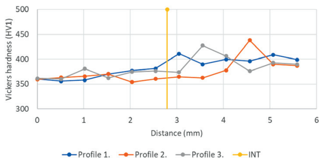
Figure 7: Vickers hardness profiles across the INT between the PBF and DED part. The PBF part present the left-hand side and the right-hand side DED part. Yellow line indicates the approximate location of the INT.
