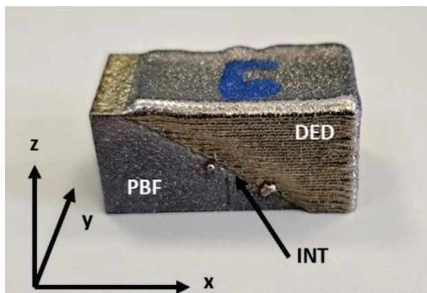
Figure 1: Photograph of finished HAM sample build by PBF and DED technology in a process chain. The INT (interface) with a black arrow shows the interface between the PBF and DED technology.
