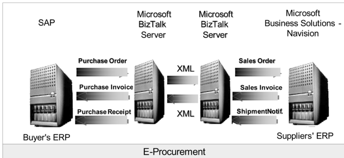
Figure 3: Case of Connecting Two Different ERP systems: Microsoft Business Solutions—Navision and SAP
