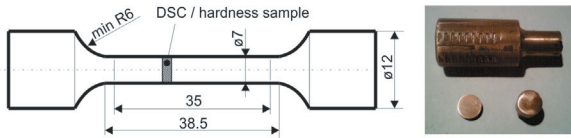
Fig. 2. Dimensions of tensile test specimens (in mm)
