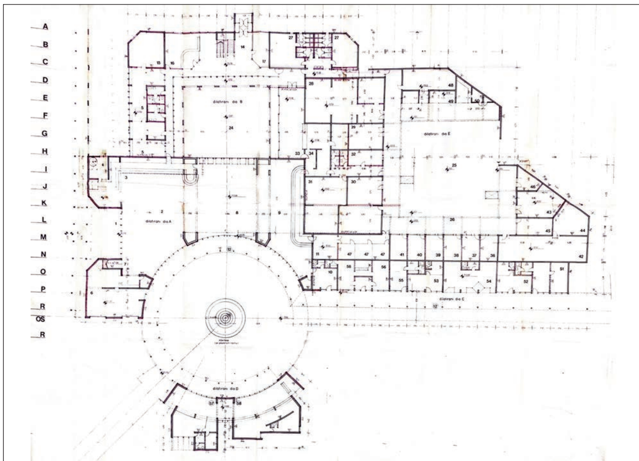
Slika 11: Prijemni terminal – Tlocrt prizemlja (DACG, 214.29). Figure 11: Reception terminal – Ground floor plan (DACG, 214.29).
