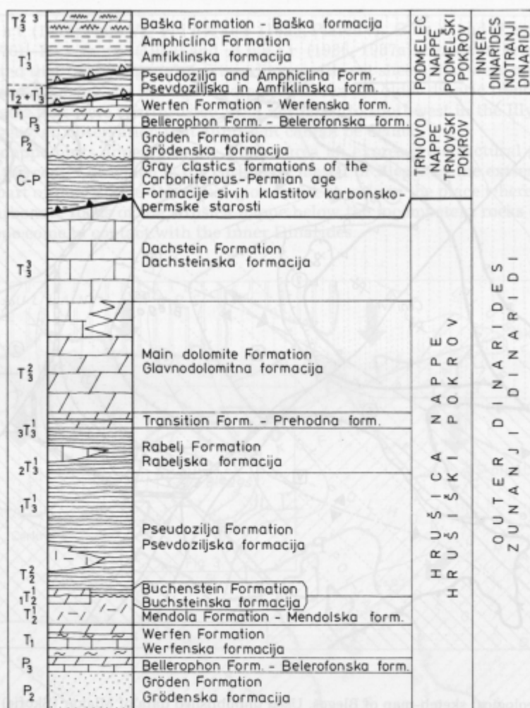
Fig. 4. Lithostratigraphic development of nappe units in the Blegoš area
