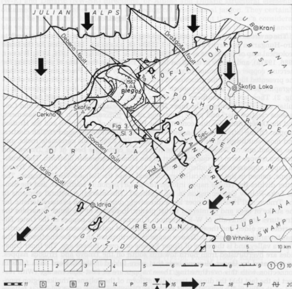
Fig. 2. Nappe subdivision of wider Blegoš surroundings
