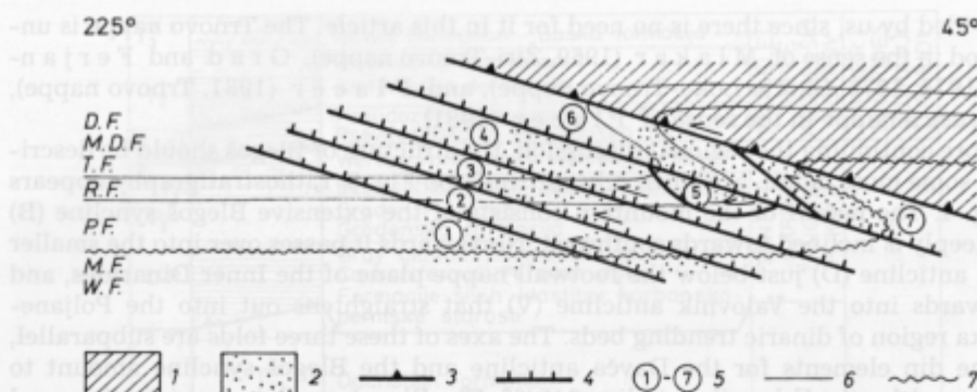
Fig. 5. Initial structure of the Blegoš horses in the Hrušica nappe
