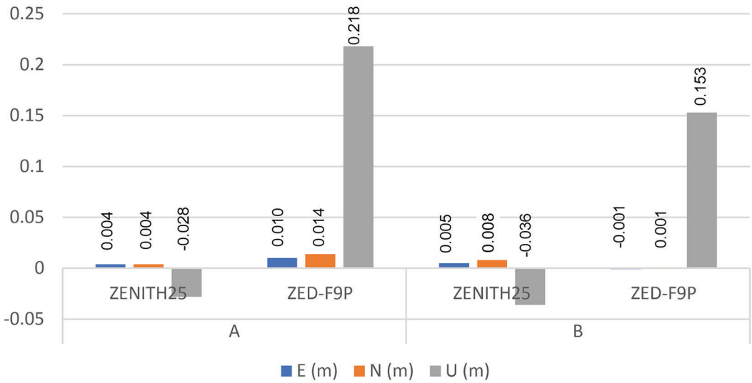
Figure 7: Differences between reference and computed coordinates expressed in Topocentric coordinates for case B.
