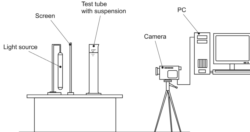
Fig. 1. Experimental setup for determination of interdependence between the age of the suspension and the settling velocity
