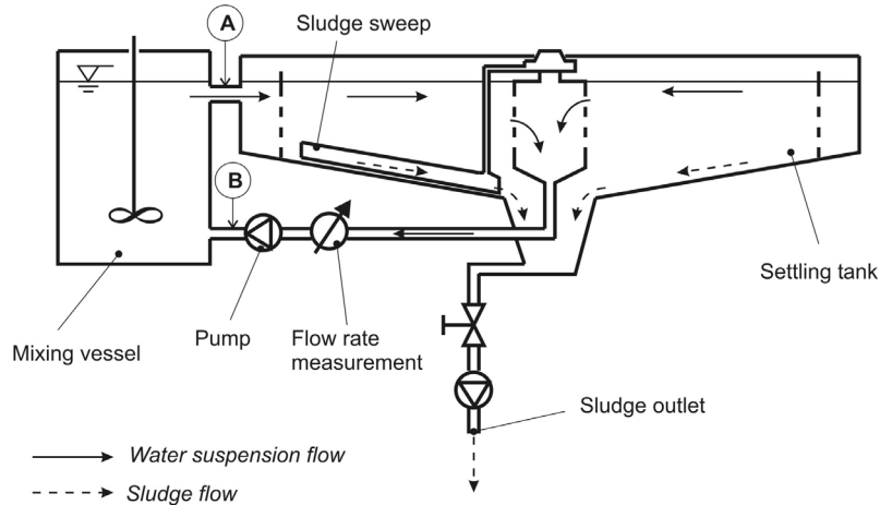
Fig. 4. Schematic view of the settling tank and water suspension/sludge flow
