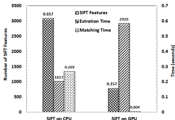
Figure 4: The evaluation of the SIFT detector on the CPU and the GPU with respect to the number of features, the extraction time, and the matching time.
