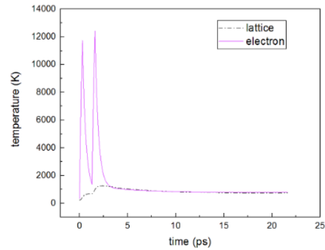
Fig. 20 Two-temperature curve under double-pulsed laser
