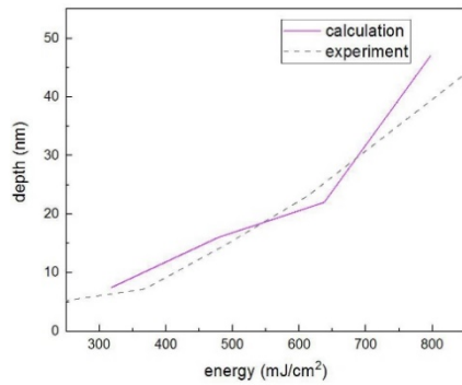
Fig. 17 Ablation depth changed by laser fluence
