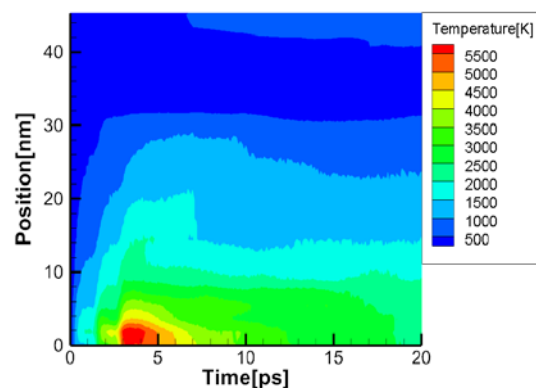
Fig. 30 Temperature contour of lattice at laser fluence of 1594 J/m 2 under multi-pulsed laser
