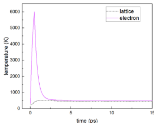
Fig. 5 Two-temperature curve with laser fluence of 1000 J/m 2 and pulse width of 500 fs
