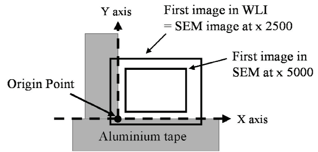
Fig. 1. Measurement methodology: drawing of a common datum, used for both techniques, on the sample surface.
