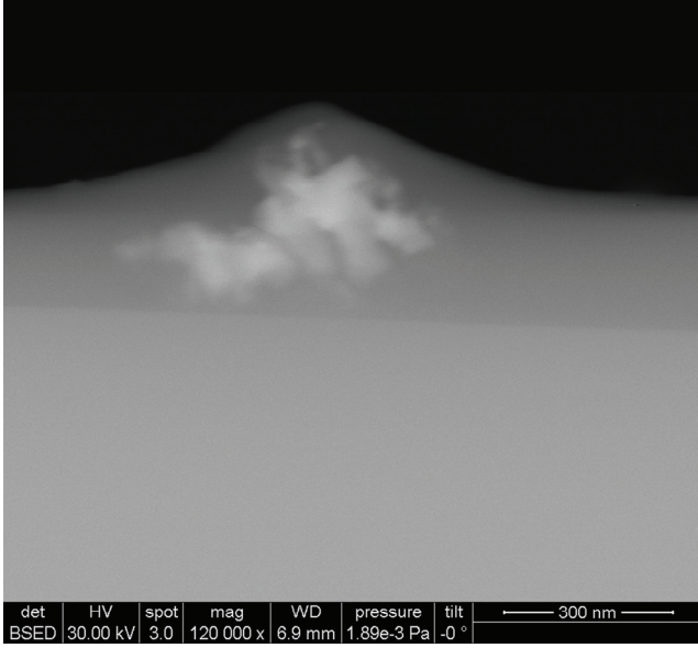
Fig. 3. Backscattered electron picture, cross-section, sample 3. The nanoparticles appear in clear white, surrounded by the polymeric matrix deposited on silicon substrate.
