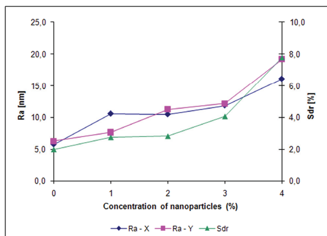
Fig. 4. Graphical representation of Ra and Sdr parameters as a function of nanoparticles concentration.
