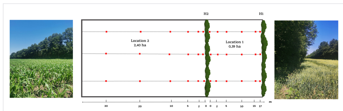
Figure 3: Location of soil sampling points in the study area
