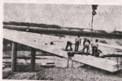
Most v km 1+045
