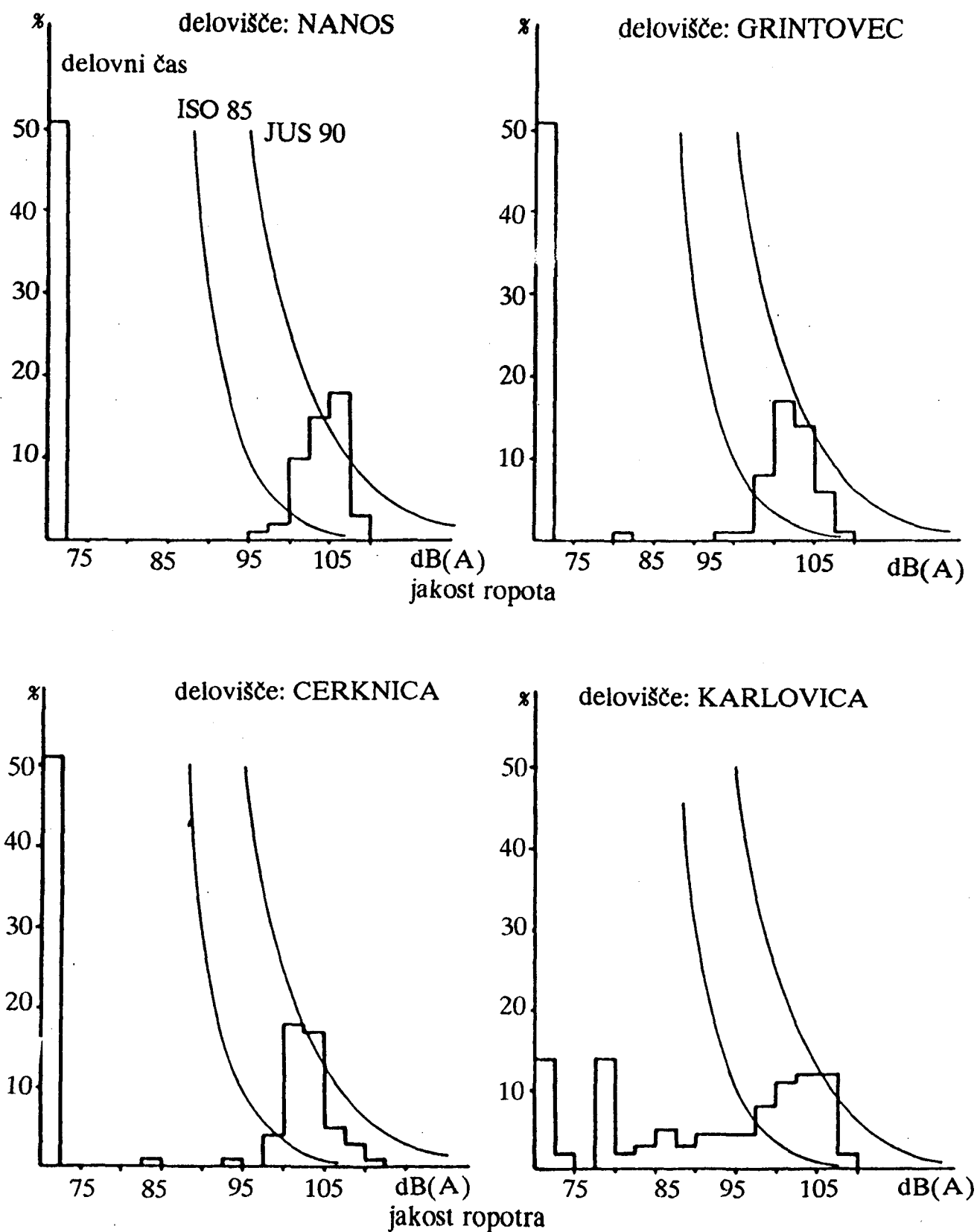
Graph 5: NOISE LEVEL FREQUENCY DURING WORKING TIME WHEN DRILLING WITH PIONJÄR 120
