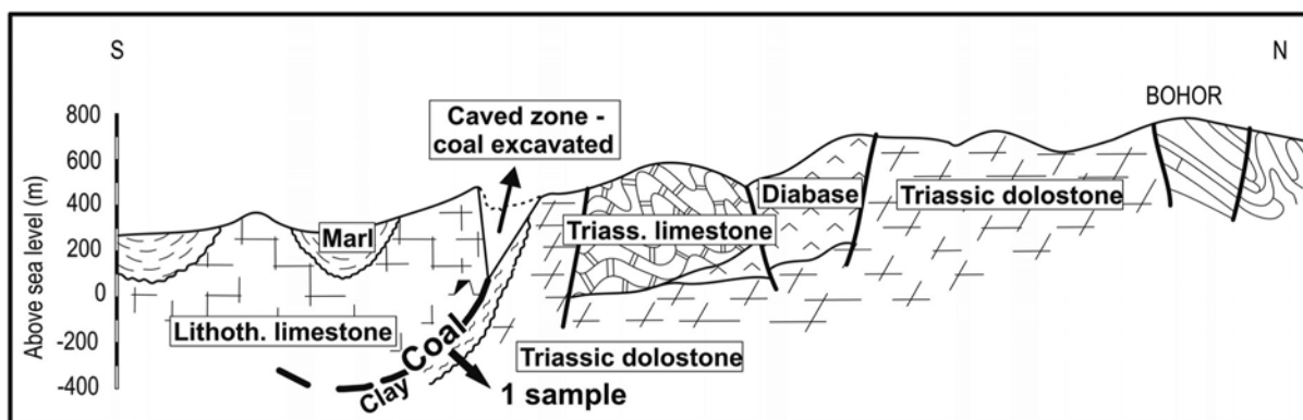
Figure 4: Geological profile of the Senovo coal deposit in N–S direction (from 16 ).
