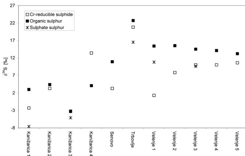
Figure 6: \delta^{34}\text{S} of different sulphur species of the studied coals.
