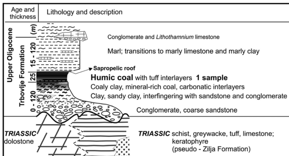
Figure 3: Lithological column of the Trbovlje coal-bearing formation of Oligocene age (based on 14 ; from 15 ).
