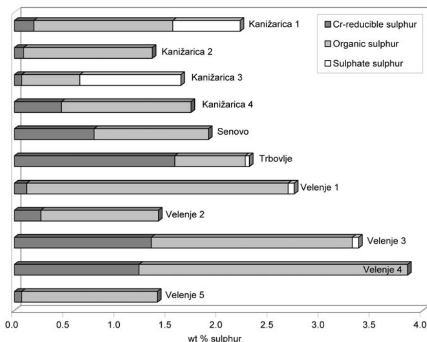
Figure 5: Composition of different sulphur species of the studied coals.
