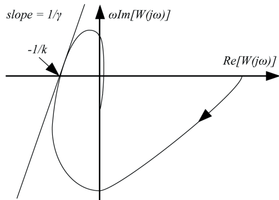
Fig. 3. Popov plot
