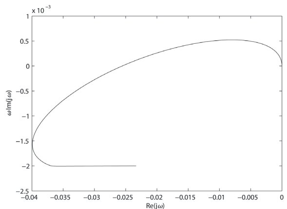
Fig. 6. Popov plot for the robustness analysis
