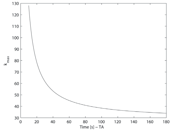
Fig. 5. Maximum allowed nonlinear gain according to the actuator delay
