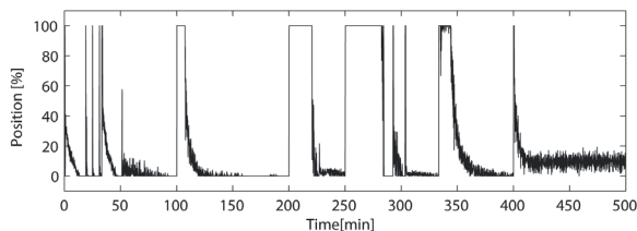
Fig. 13. Position of the continuous valve (PI)
