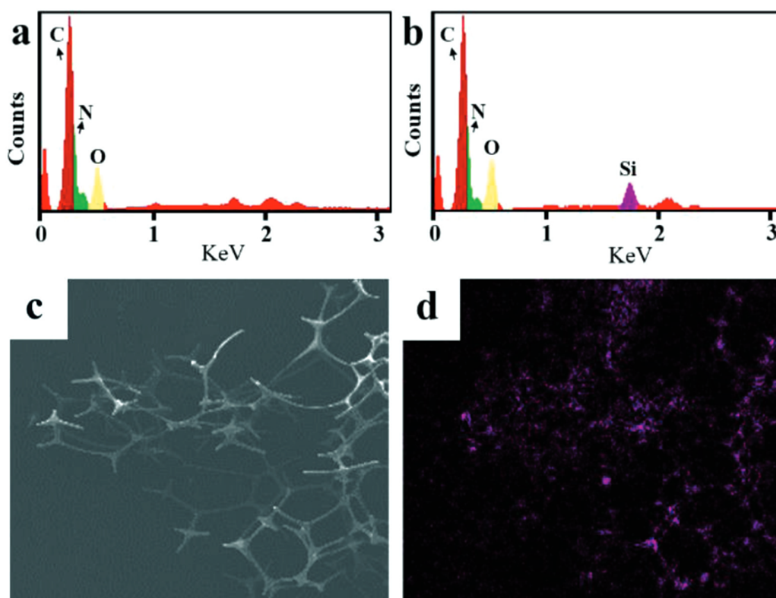
Figure 2: EDS diagrams of: a) unmodified sponge, b) modified sponge and c, d) mapping diagrams of modified sponge
