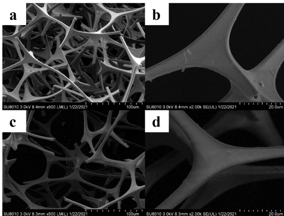
Figure 1: SEM photos of sponge samples: a, b) unmodified sponge and c, d) modified sponge
