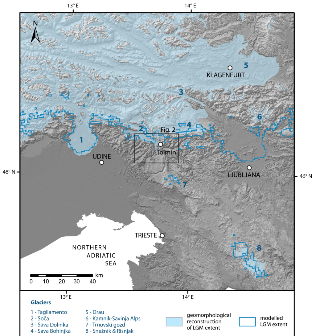
Fig. 1. LGM glacier extent in southeastern European Alps. The extent of the modelled LGM glacier driven by the EPICA paleo-temperature record and paleo-precipitation correction is after Seguinot et al. (2018), while the geomorphological reconstruction of the extent of the LGM glacier is modified from Ehlers et al. (2011). The digital terrain model is from SRTM data (Shuttle Radar Topography Mission), accessible from EarthExplorer ( https://earthexplorer.usgs.gov/ ).
