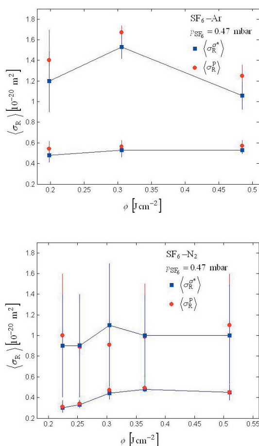
Figure 5. Average bulk rotational relaxation cross sections, \langle \sigma_R^{\sigma^e} \rangle , in SF 6 -Ar and SF 6 -N 2 gas mixtures as a function of laser fluence. Average values obtained from the “point” methods \langle \sigma_R^P \rangle for different gas mixtures are also presented.
