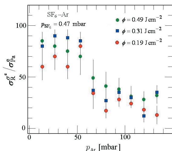
Figure 6. The ratio of bulk rotational cross-section \sigma_R^{\sigma^e} and enhanced absorption cross-section, \sigma_R^{AB} , as a function of buffer gas pressure for different laser fluences.
