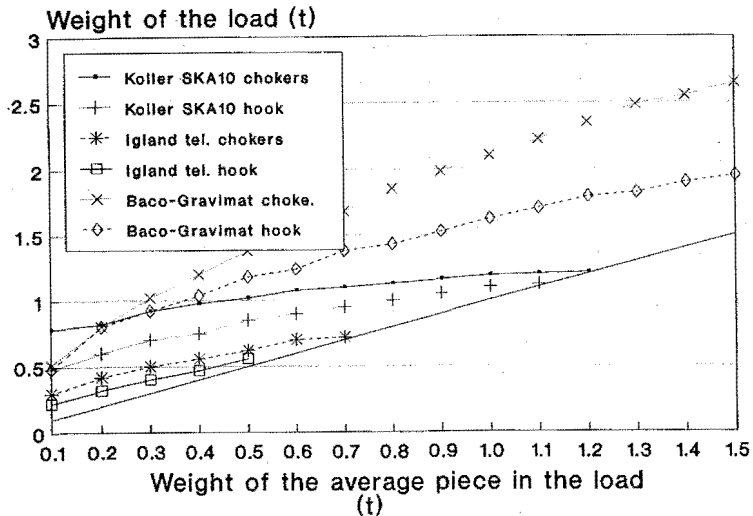
Figure 3: The load weight dependence upon a single-log weight and upon the style of wood fastening
