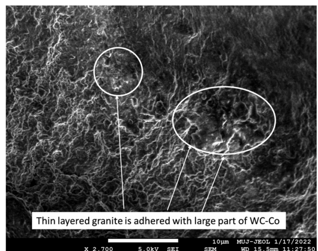
Figure 7: Granite-layer formation over the surface of WC-Co surface
