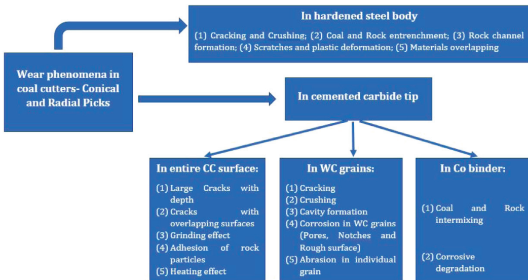
Figure 2: Flow chart showing detailed wear phenomena in coal cutters
