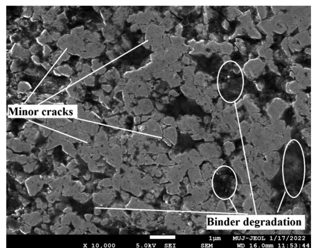
Figure 4: Minor crack generation in WC grains
