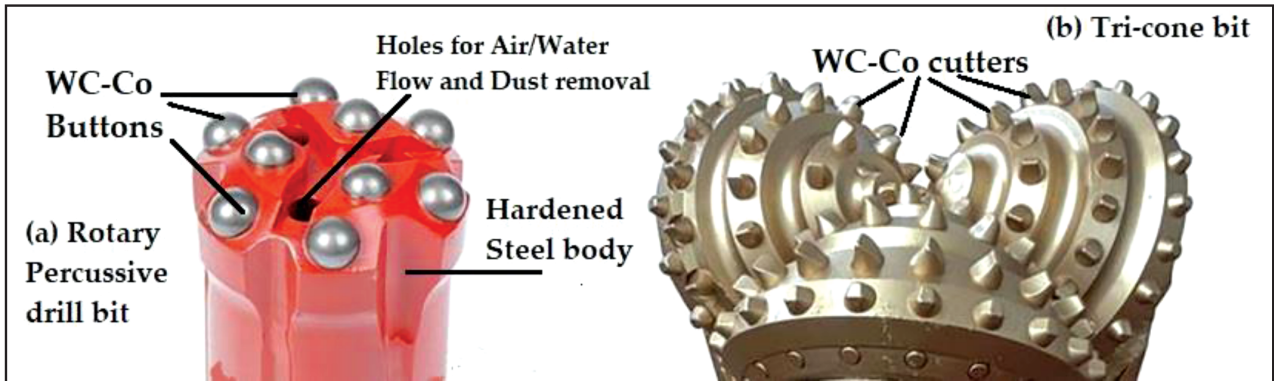
Figure 1: a) Rotary percussive drill bit with WC-Co buttons inserted by brazing method, 2 b) Tri-cone bit with WC-Co cutters 3
