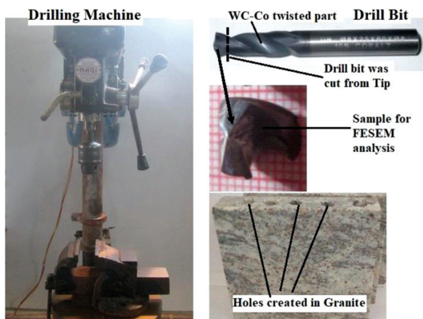
Figure 3: Experimental set-up
