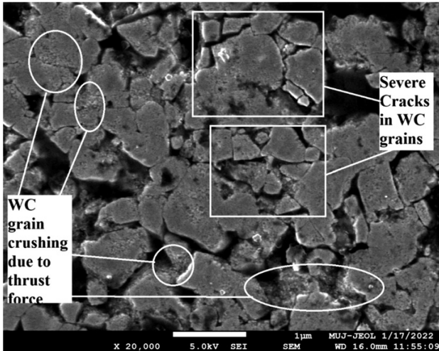
Figure 5: Severe cracks and Crushing of WC grains
