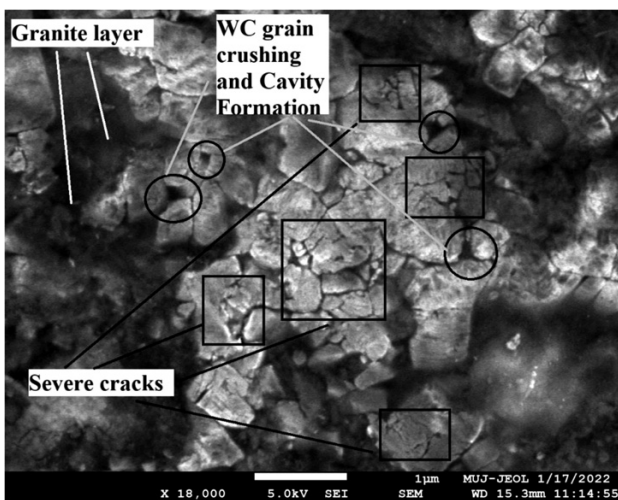
Figure 6: Severe cracks and cavity formation in WC grains; binder parts are surrounded by granite particles, forming a layer of rock
