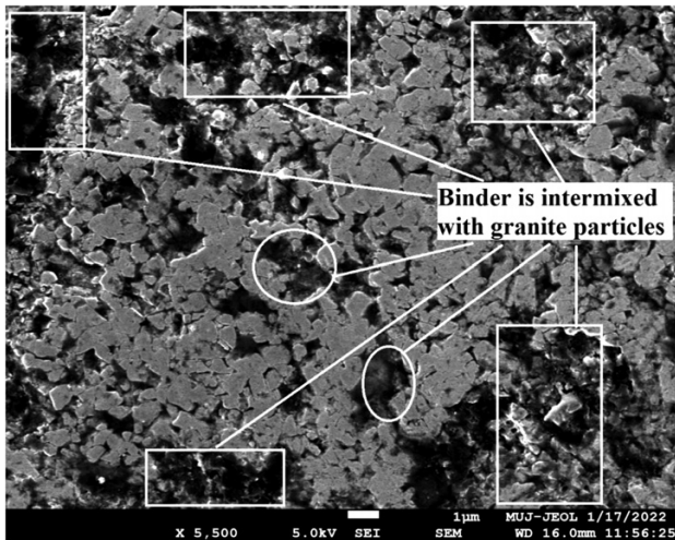
Figure 8: All rectangular and circular areas are showing Co-binder intermixed with granite particles
