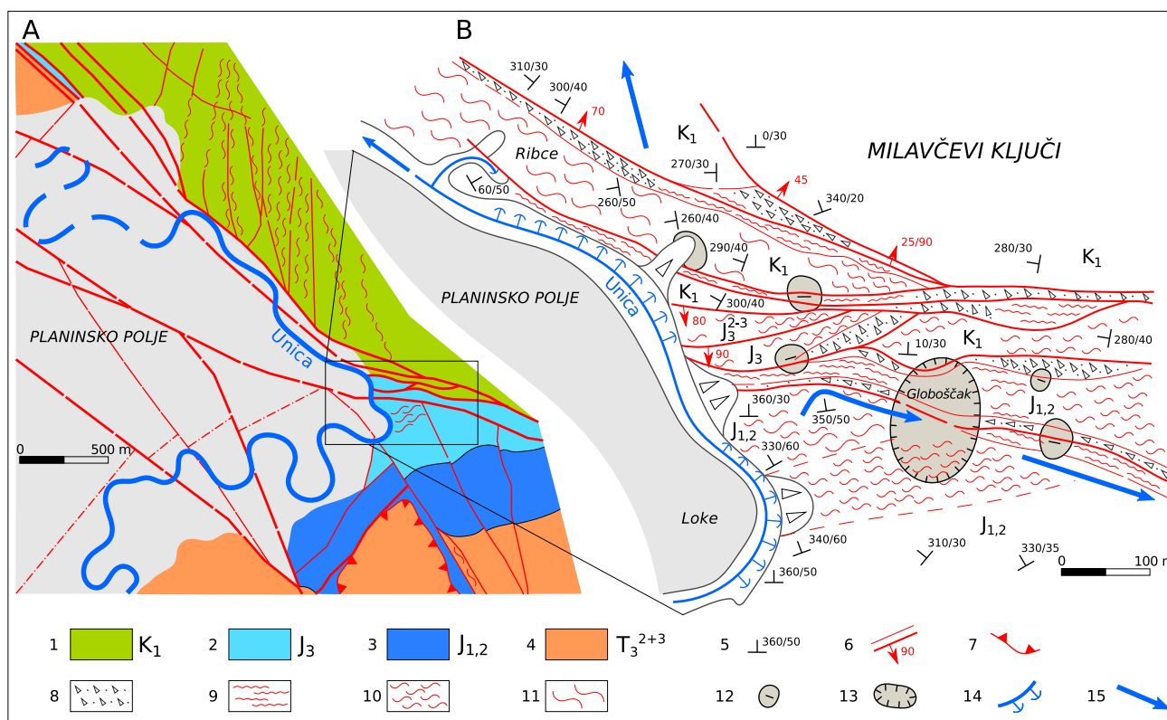
Fig. 11. Drawings A and B: General geological and hydrological situation in the area of Milavčevi ključiči at Planinsko polje. Drawing A: Geological situation at the Milavčevi ključiči ponor zone.
