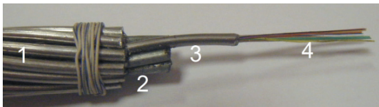
Fig. 1. a) Cross sectional view of OPGW; b) view of OPGW; (1) AA6101, (2) steel wire, (3) steel tube, (4) fibres
