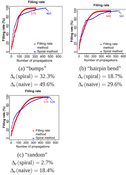
Fig. 8. Comparison of the filling rates \tau of the distances array, between the method based on the filling rate of the distances array (in red) and the spiral method (in blue) for the images "bumps", "hairpin bend" and "random". The relative differences \Delta_r(\text{spiral}) (resp. \Delta_r(\text{naive}) ) of the number of propagations of the method based on the filling rate compared to the number of propagations of the spiral (resp. naive) method are given on the bottom lines.
