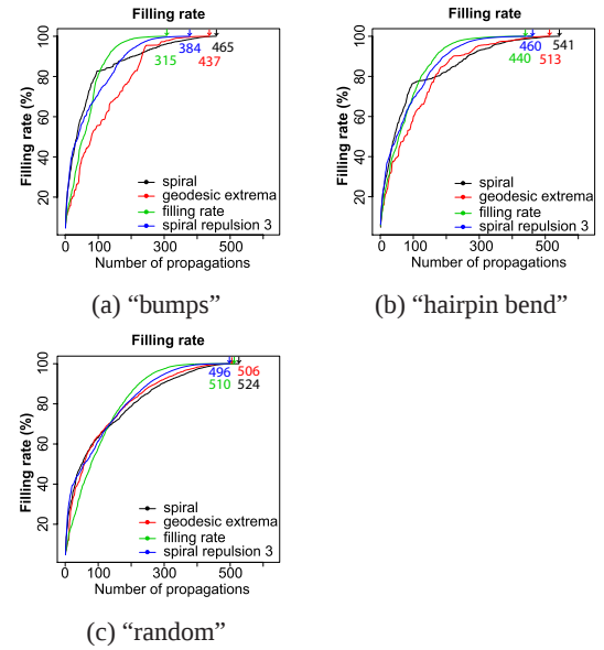
Fig. 9. Comparison of the filling rates, of the array of distances, for the methods: spiral, geodesic extrema, the method based on the filling and the spiral method with a repulsion distance of 3 pixels for the images "bumps", "hairpin bend" and "random".
