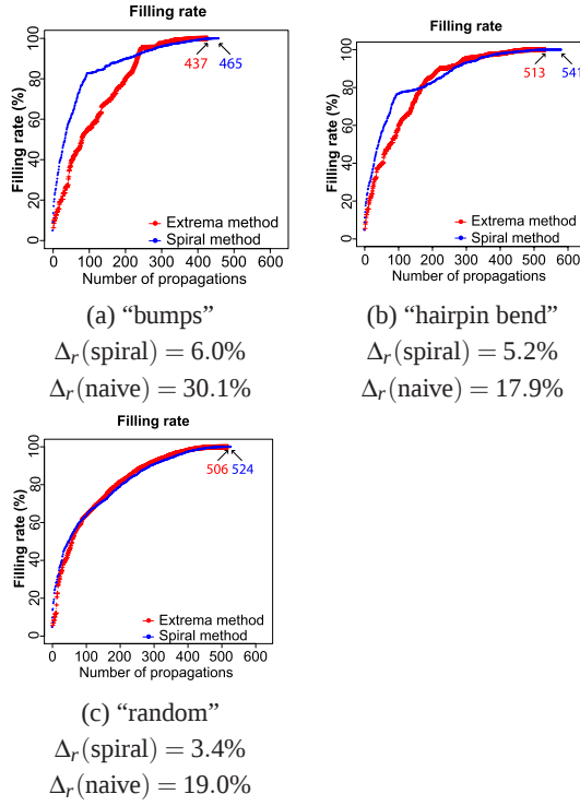
Fig. 7. Comparison of the filling rates \tau of the distances array, between the geodesic extrema method (in red) and the spiral method (in blue) for the images “bumps”, “hairpin bend” and “random”. The relative differences \Delta_r(\text{spiral}) (resp. \Delta_r(\text{naive}) ) of the number of propagations of the the geodesic extrema method compared to the number of propagations of the spiral (resp. naive) method are on the bottom lines.
