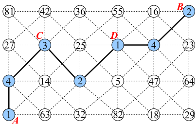
Fig. 1. Discrete geodesic path on a 8-neighborhood graph. The points C and D belong to a geodesic path between A et B . Therefore the geodesic distance between C and D is also known.
