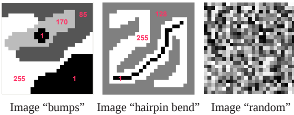
Fig. 2. Images of size 25 \times 25 pixels “bumps”, “hairpin bend” and “random” whose grey levels are between 1 and 255.
