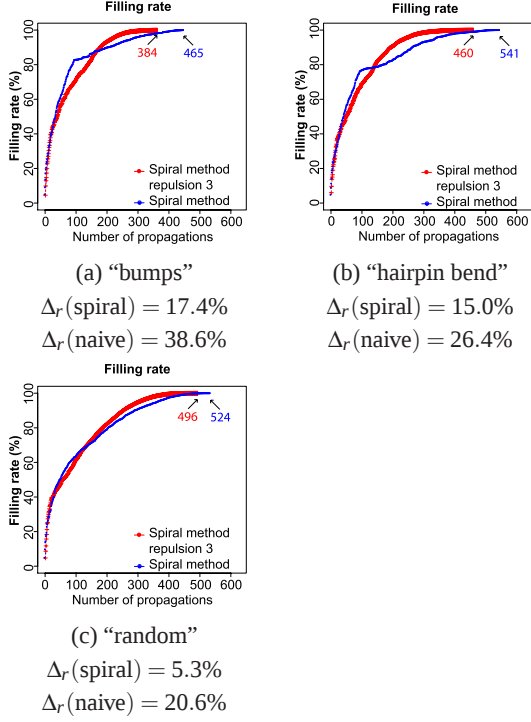
Fig. 5. Comparison of the filling rates \tau of the distances array, between the spiral method with repulsion (in red) and the spiral method (in blue) for the images “bumps”, “hairpin bend” and “random”. The relative differences \Delta_r(\text{spiral}) (resp. \Delta_r(\text{naive}) ) of the number of propagations of the spiral method with repulsion compared to the number of propagations of the spiral (resp. naive) method are given on the bottom lines.
