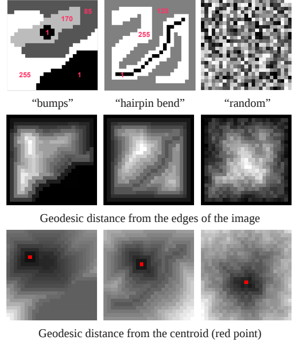
Fig. 6. Geodesic distance from the edges of the image (second line) and from the centroid in red (third line) for several images.
