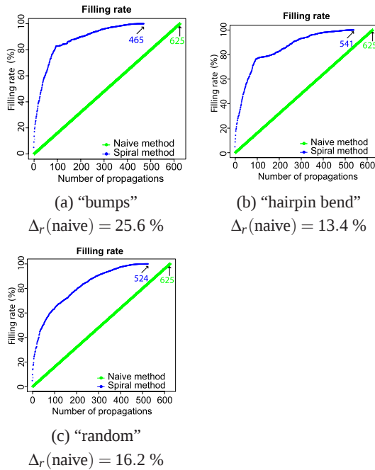
Fig. 4. Comparison of the filling rates \tau of the distances array, between the naive method (in green) and the spiral method (in blue) for the images “bumps”, “hairpin bend” and “random”. The relative differences \Delta_r(\text{naive}) of the number of propagations of the spiral method compared to the number of propagations of the naive method are given on the bottom line.
