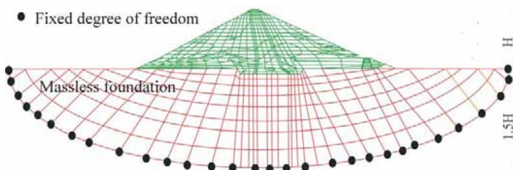
Figure 5. Rock massless model, section YI=150 m.
