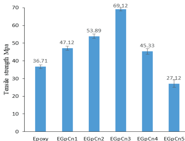
Figure 3: Tensile strength of epoxy and its hybrid nanocomposites
