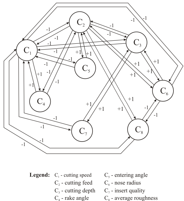
Fig. 1. NPN logic-based FCM of the machining parameters
